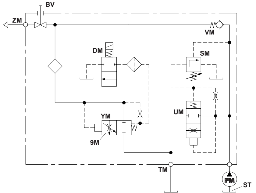
Hydraulic Circuit
